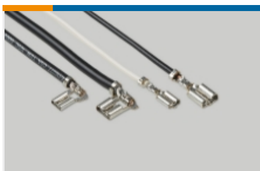
Quick Disconnects(189)
